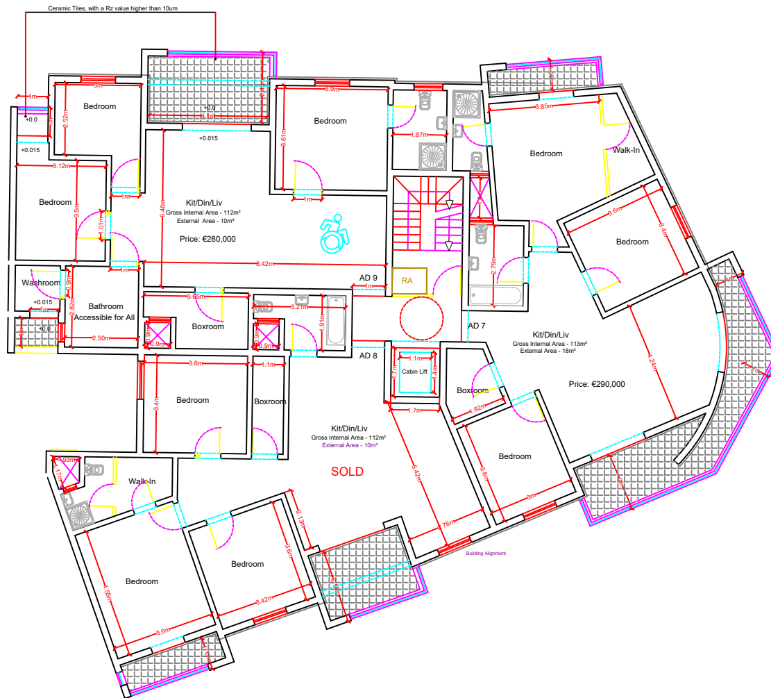
Approved/ Proposed Level 2 Scale 1:100
