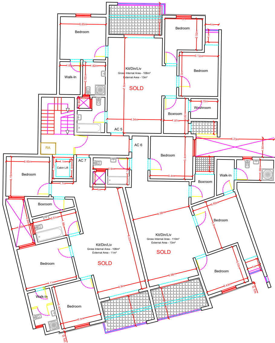
Approved/ Proposed Level 2 Scale 1:100
