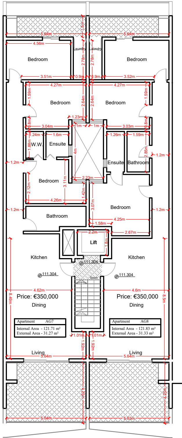
PROPOSED PENTHOUSE PLAN Scale 1:100
